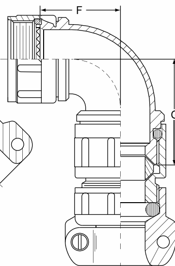
90° ENTRY ROTATABLE COUPLING 2M390MA077
